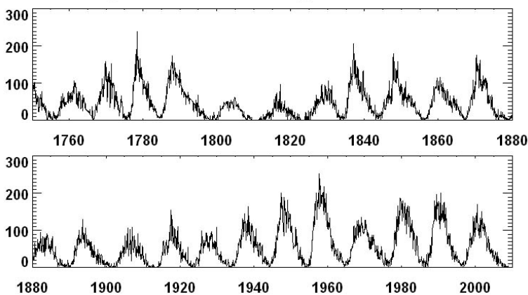
Sunspot Count: 1745 through December 2009
