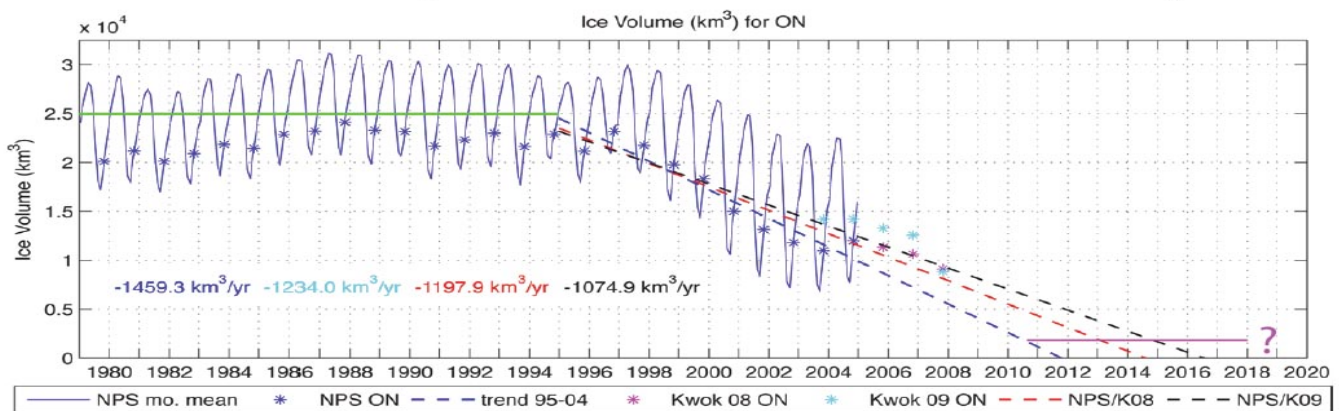
Modeled monthly mean sea ice volume (blue line) over the Arctic Ocean for the period '79-'04. Green line is the mean model ice volume for '79-'95. Stars show minimum October-November values from model (blue) and observational estimates (magenta (Kwok and Cunningham, 2008) and cyan (Kwok et al., 2009)). Red and black dashed lines: Calculated (NPS/K08 and NPS/K09) linear trend through '95-'07. Blue dashed line: Model trend through '95-'04. Projecting the trend into the future indicates that autumn could become near ice free between 2011 and 2016 (Maslowski, 2009) Purple line: An unknown minimum amount of ice volume expected to survive summer melt beyond that time.
